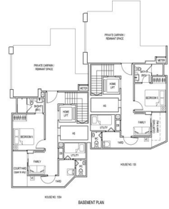
BASEMENT PLAN
